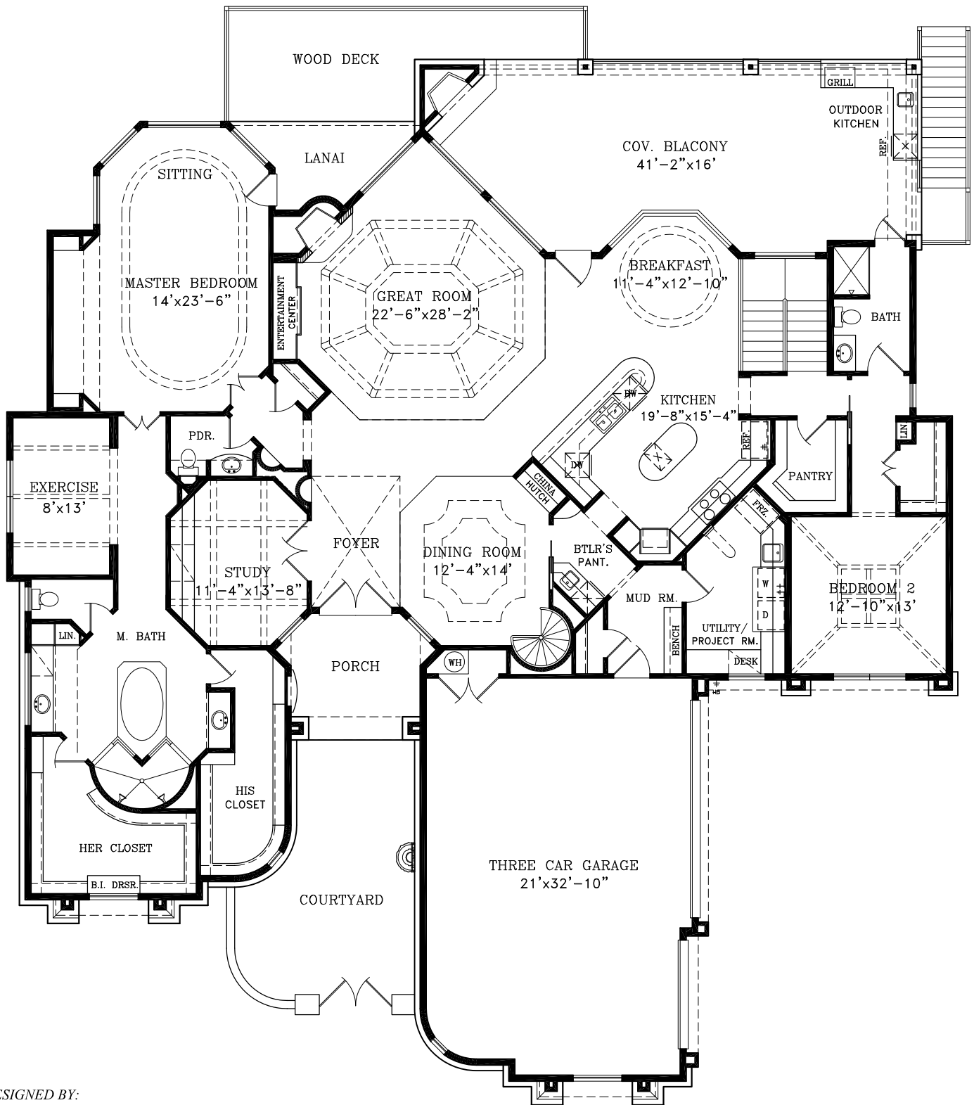
SECOND (MAIN) FLOOR
